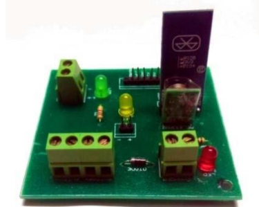
Fig. 6. PBC of controller of Underwater Robot (command transmitting part)
